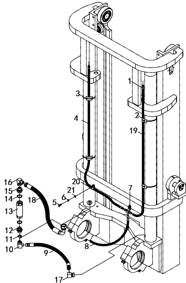
图 15 管路系统 Fig.15 Lifting oil circuit
