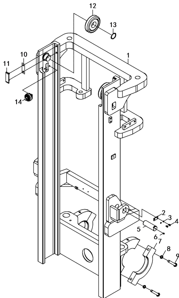
图 24 外门架 Fig.24 Outside mast
