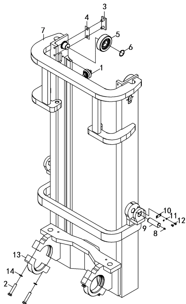
图1 外门架 Fig.1 Outside mast
