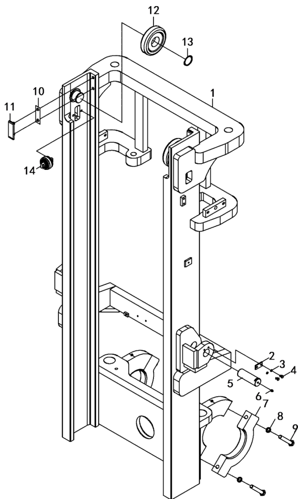
图 17 外门架 Fig.17 Outside mast
