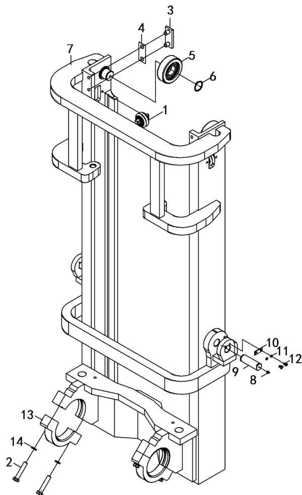
图 8 外门架 Fig.8 Outside mast
