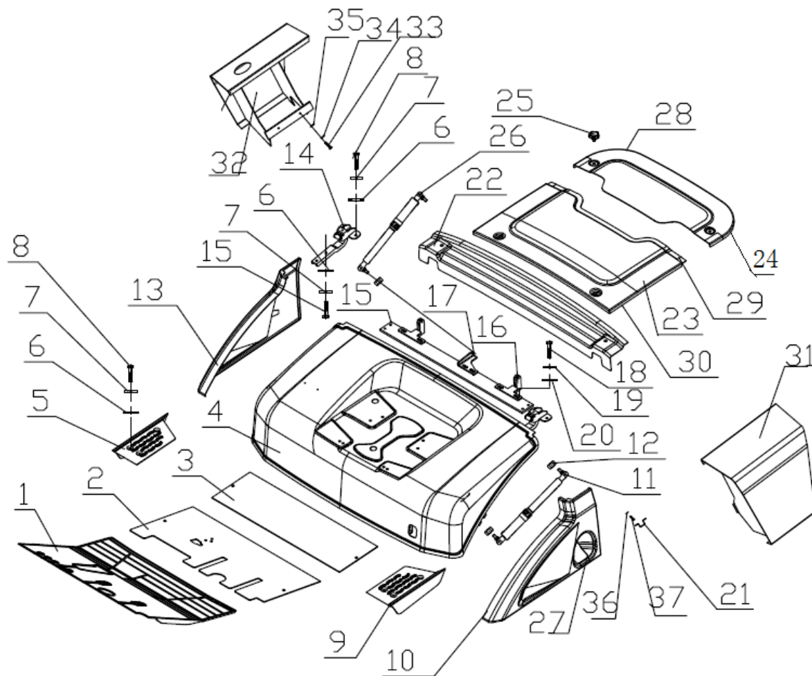
图6 机罩及底板总成 Fig.6 Hood and floor board assy
